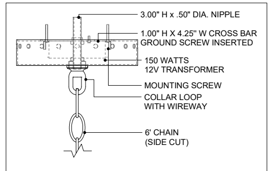
CANOPY DETAIL
